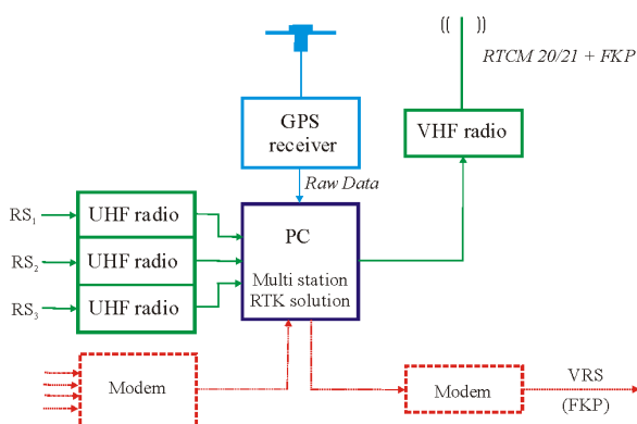
Figure 6: Hardware set-up for the RTK network processing centre
