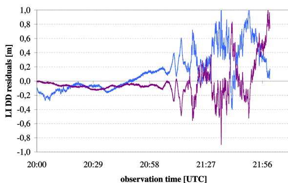
Figure 12: LI DD-Residuals during sunset (UFPE-TELE (15 km), SV 3-1, 3-31)
