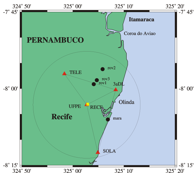
Figure 4: GPS reference network Recife with the coastline of Pernambuco. The RBMC station (square), reference sites (triangles), and permanent rover (circles) are plotted. The large circle with 20 km radius represents an hypothetical area of equal accuracy of better than 5 mm.
