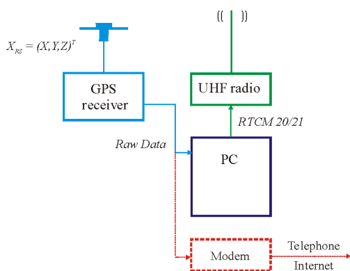
Figure 5: Reference station equipment
