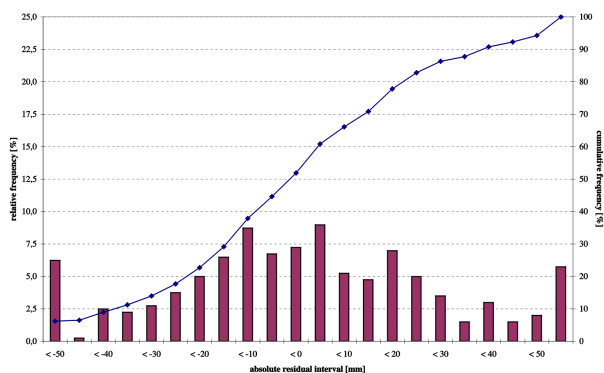
Figure 9: Vertical positioning accuracy
