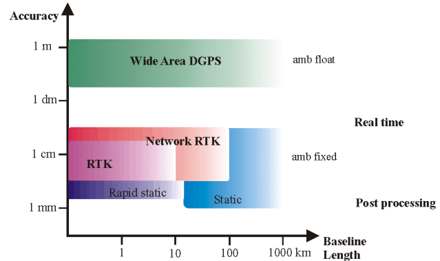
Figure 2: Range dependent accuracy of different GPS positioning methods
