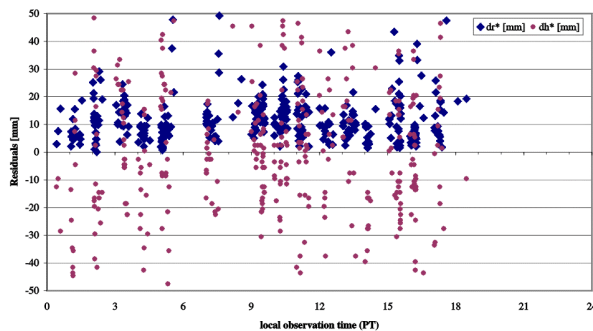
Figure 11: Availability and accuracy of RTK network solutions depending on local observation time
