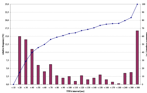
Figure 10: Time to fix ambiguities (TTFA)
