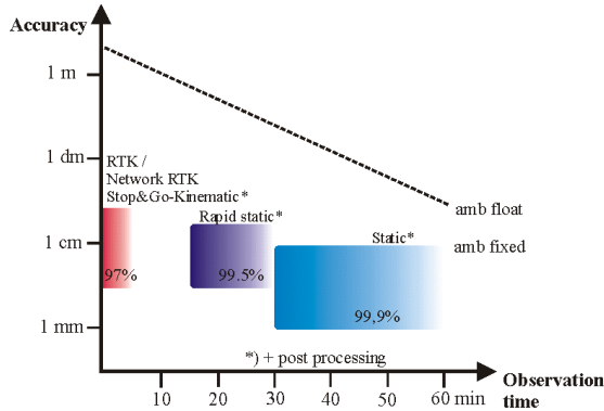
Figure 1: Obtainable accuracy and reliability depending on observation time and positioning method
