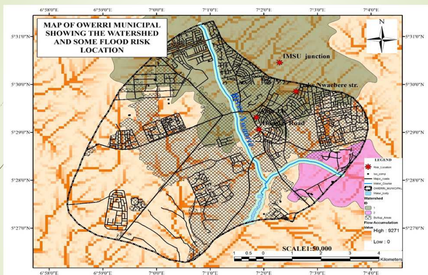
Fig. 5 Map of Owerri Municipal showing the watershed and risk location Source: Digitized from the SPOT5 satellite image covering the study area
