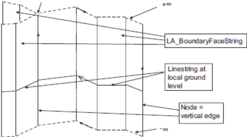
Figure 6. Boundary face string concepts (ISO, 2012)
