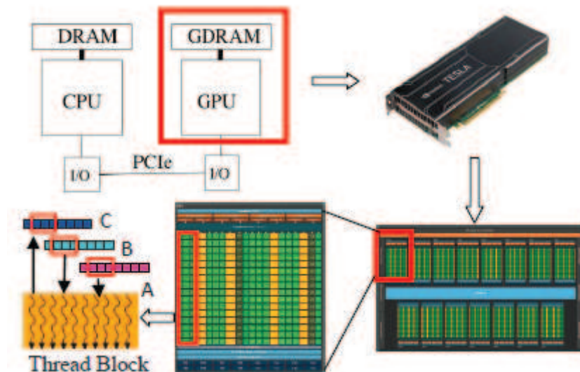
Figure 14. Illustration of GPU hardware Architecture (according to (Zhang et al, 2015c))
