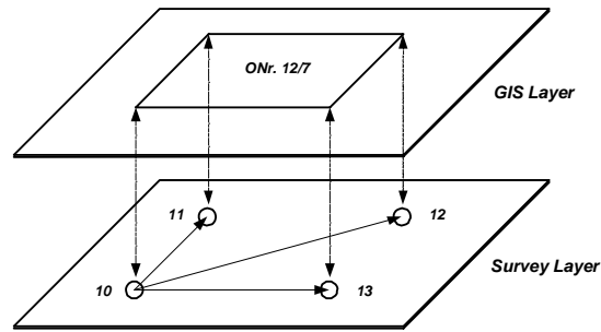
Figure 5: The link between survey and GIS data
